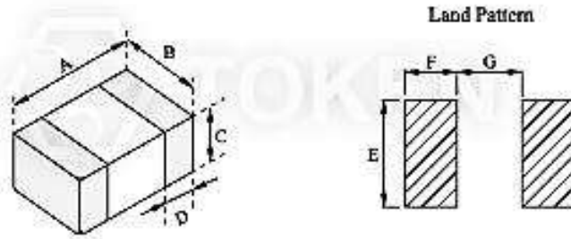
RF Surface Mount (TRMF) Dimensions
