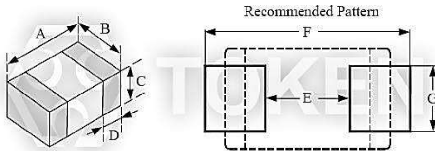
(TRMB) Recommended Pattern and Dimensions (Unit: mm)
