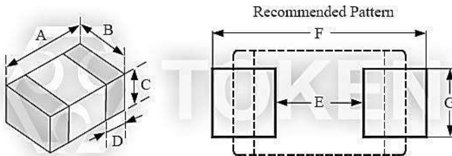
(TRMA) Recommended Pattern and Dimensions
