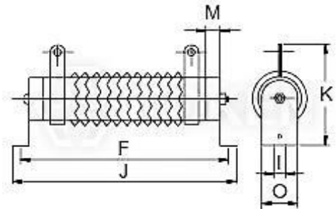
(DQ-A) G - Horizontal Mount
