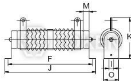
(DQAN) G - Horizontal Mount
