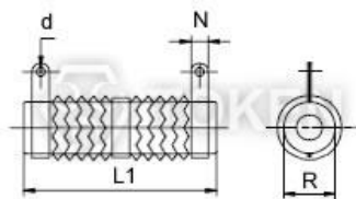
(DQBN) N - No Mount
