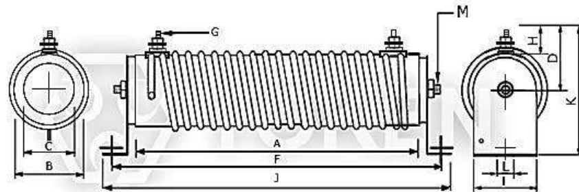
Power Starter (DST 600W ~ 1000W) Dimensions
