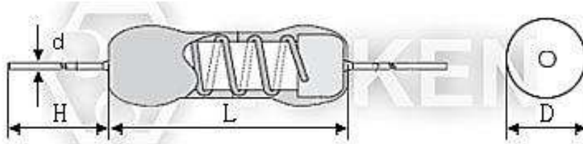
Wire Wound (KNP) Dimensions (Unit: mm)
