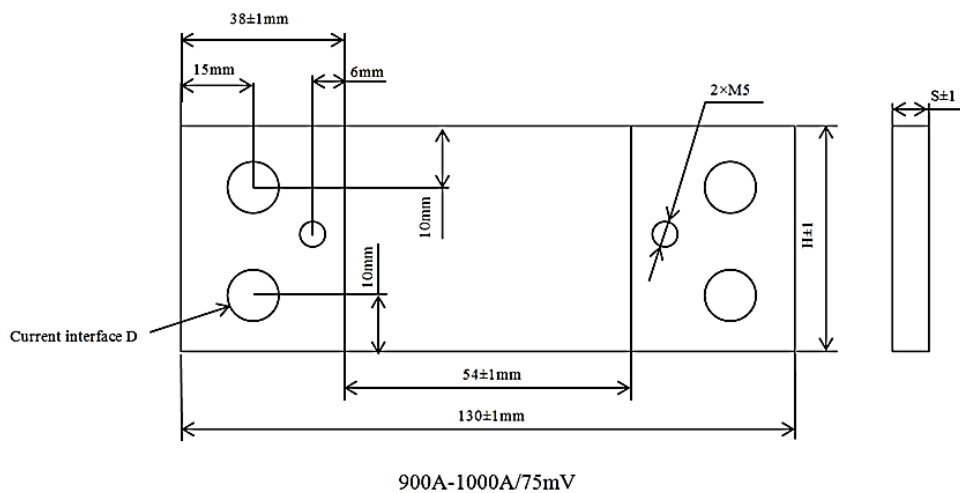
Electron Beam Welding Precision Shunt Dimensions (Unit: mm)
